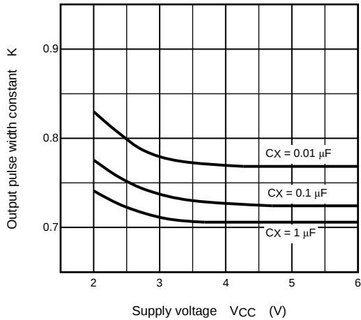
Output Pulse Width Constant K – Supply Voltage (typ.) (external resistor (R X ) = 10 kΩ: t wOUT = K·C X ·R X )
